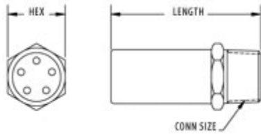
Female – 1/8"- 1/2"
