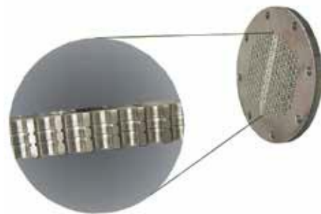
Grooved Tubesheets
