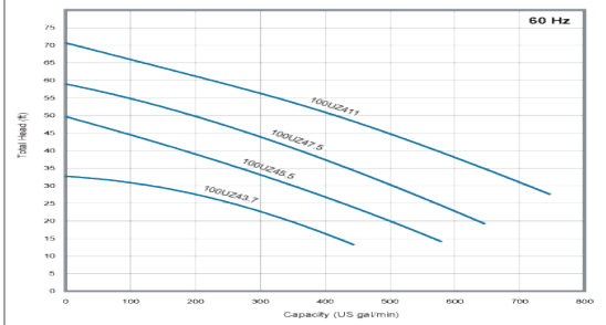
UZ SERIES PERFORMANCE RANGE 3.94" (100 mm) SOLIDS HANDLING
